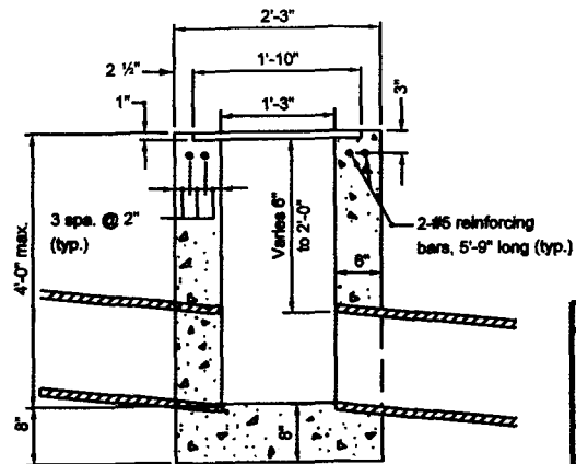
SECTION D-D TYPE T
