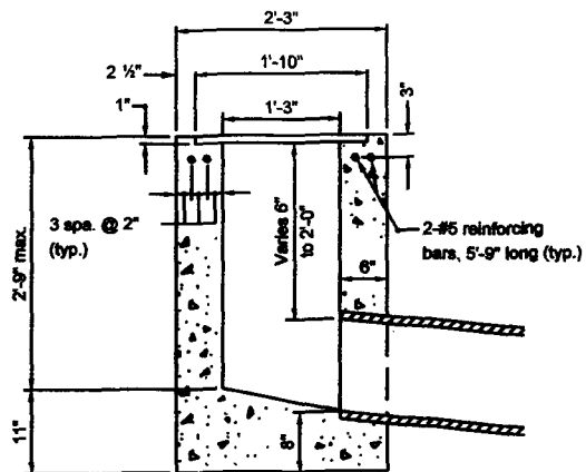
SECTION C-C TYPE S
